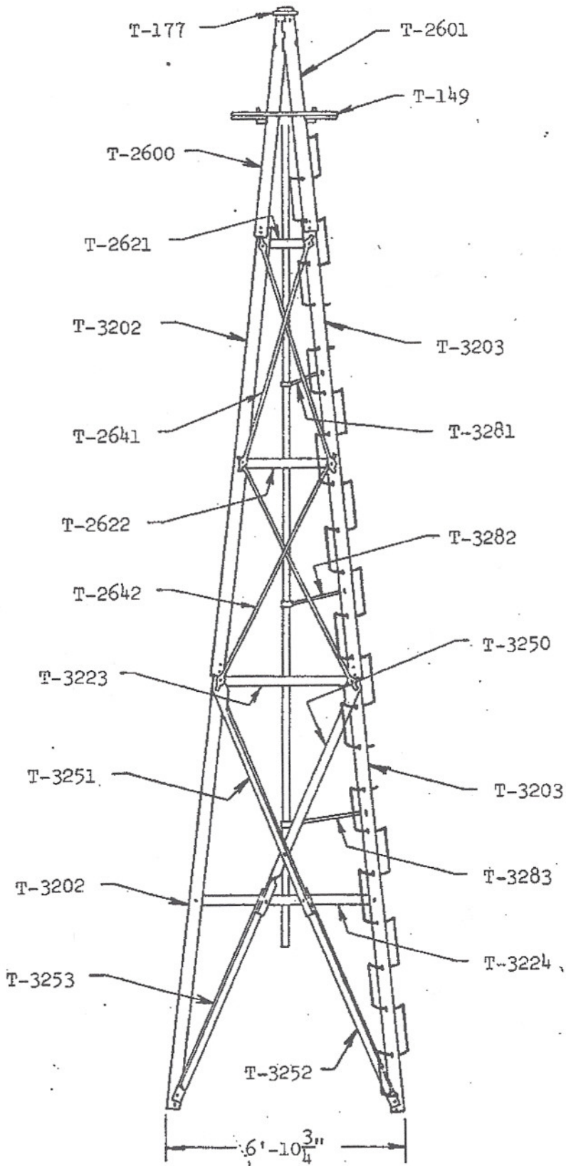
33 FT. 4 POST TOWER FOR 6 OR 8 FT. MILL
