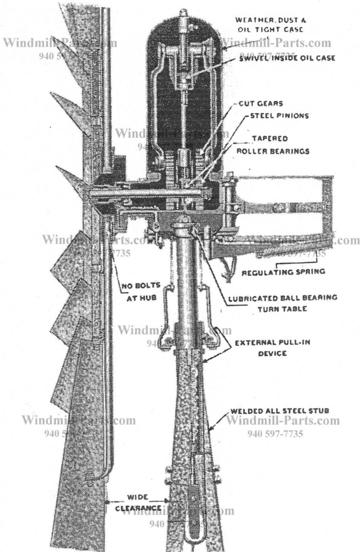
Cross Section View of Reatty Pumper
